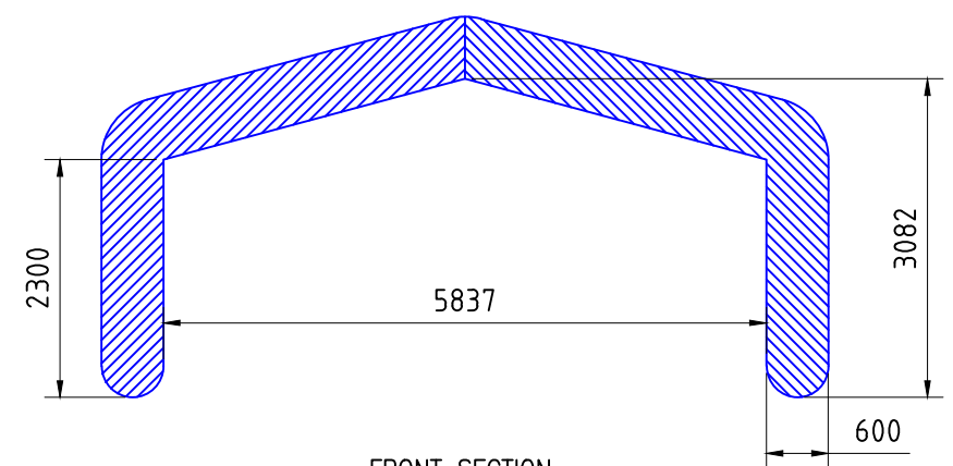
FRONT SECTION
